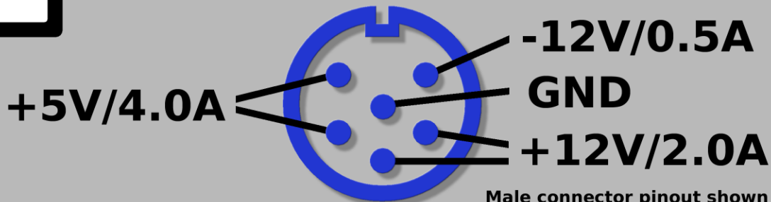
Male connector pinout shown on drawing
