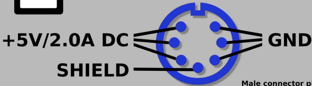
Male connector pinout shown on drawing
