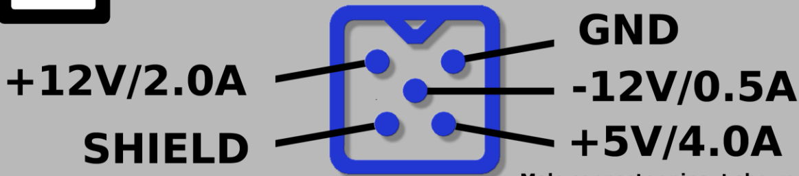
Male connector pinout shown on drawing
